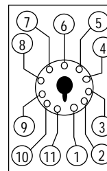
Terminal Arrangements (top view)
